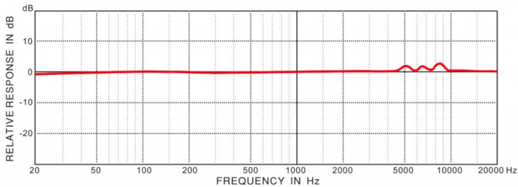
Behringer ECM8000 Official Frequency Response
